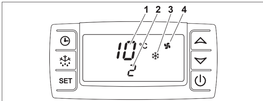
Figure 7: Temperature indication
